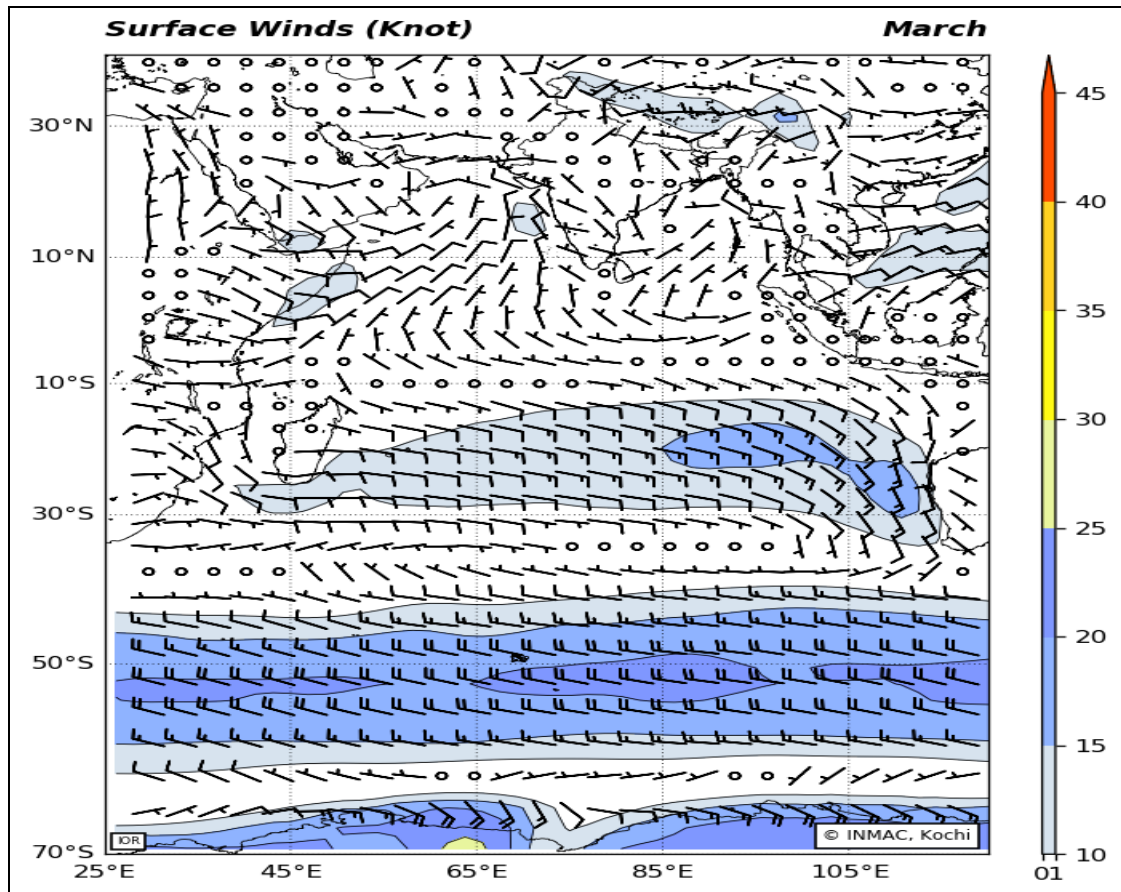
Fig 2. Surface Wind and Direction (Kt) over IOR - Mar
